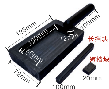
KYG0665 翻沙油槽 Ingot Mould Weight:1.53kg
