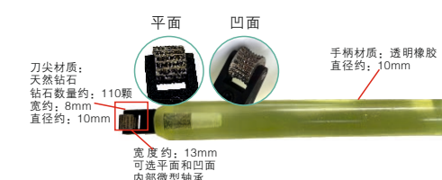
KYG0176 滚砂棒 Sand Rolling Needle 126粒砂 Size: \phi 12 \times 210 mm
