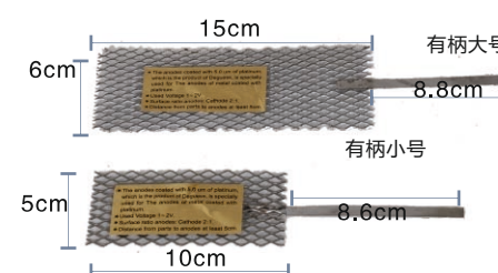
KYG0486 国产钛网 Titanium Mesh Size:5 × 10cm Size:6 × 15cm Made in China
