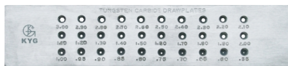
KYG1148 六角型(30孔)Hexagonal—30 holes No.0.55-3.00 Size:208×46×7.5mm
