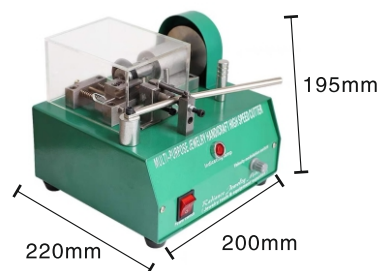
KYG0319 多功能切割机 Multifunctional Cutting Machine 空载转速No-Load Speed: 6800RPM 额定电压Rated Voltage: 110V-220V 切割能力Cutting Ability: 金属切割Metal cutting 额定功率Rated Power: 360W 产品净重Product Net Weight: 5.6kg
