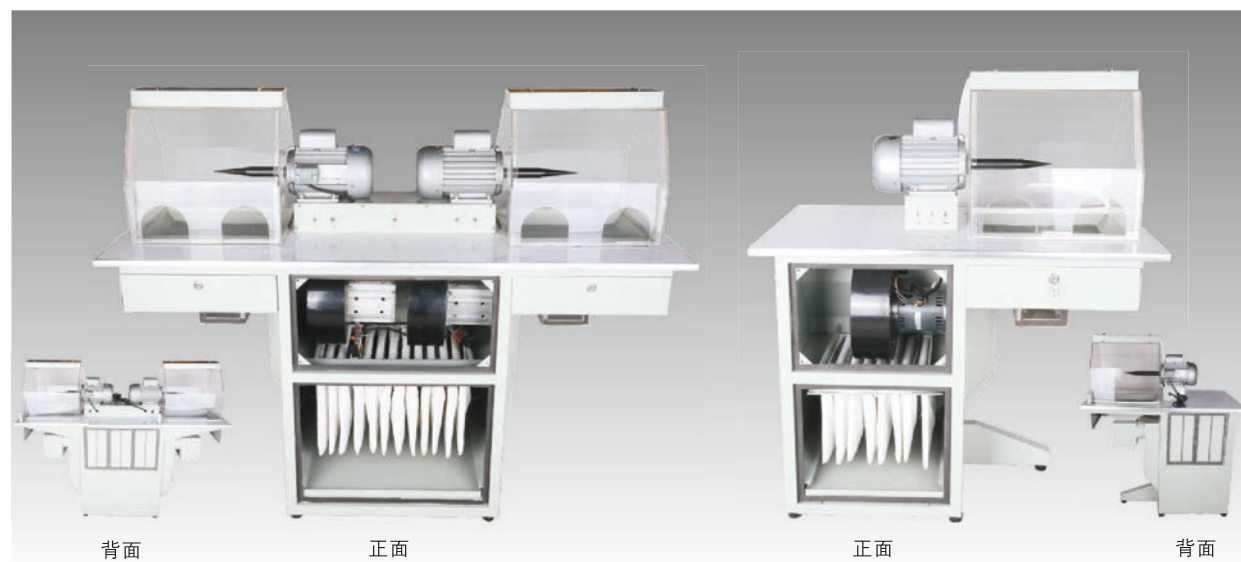
KYG0760 双位吸尘打磨机 Polishing Machine With Mute Dust Collector 2 Motors 电压(Voltage): 220V 功率(Power): 550W × 2pcs 吸尘功率(Dust Suction Power): 550W × 2pcs 转速(Rev): 2800RPM Size: 1500 × 610 × 1200mm Weight: 110kg
