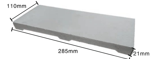
KYG1541 优质陶土六脚焊瓦 Sintering Refractory Tile--Large Size: 110x285x21mm
