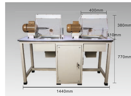
KYG0764 双位吸尘打磨机 Double Ended Polishing Machine 打磨功率Power: 550W × 2 吸尘功率Polishing power: 1100W 电压Voltage: 220V 重量Weight: 109kg
