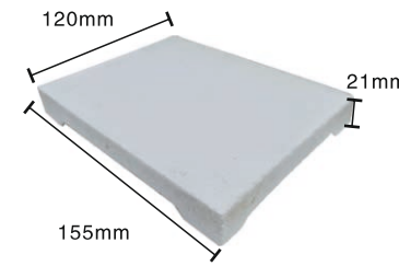
KYG1539 石英四脚焊瓦 Sintering Refractory Tile--Small Size: 120x155x21mm
