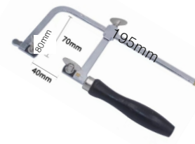
KYG1007 黑柄锯弓(活动) Saw Bow Adjustable Outlook Size:80 × 195mm Made in China
