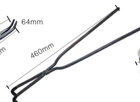
KYG0679 坩埚钳 Crucible Tong Weight:520g
