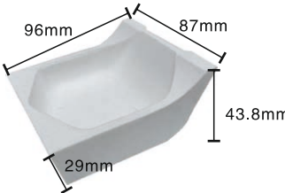
KYG1526 石英坩 Ceramic Melting Crucible Size:96x87x43.8mm
