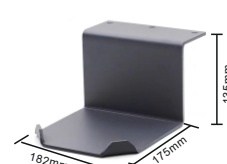
KYG0130 简易型承铁 Large Block Shelf 铁厚度Iron thickness:5mm 重量Weight:2.65kg
