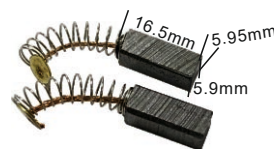
KYG0032 保利达摩打碳刷 Pflingst Carbon Brush 长度Length: 5.5 x 5.9 x 16.5mm 重量Weight: 3g
