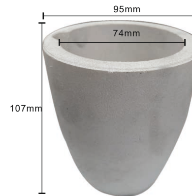
KYG1546 石英熔金坩 Ceramic Melting Crucible
