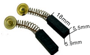
KYG0031 金科达摩打碳刷 Foredom Carbon Brush 长度Length: 5.5 x 5.9 x 18mm 重量Weight: 3.2g
