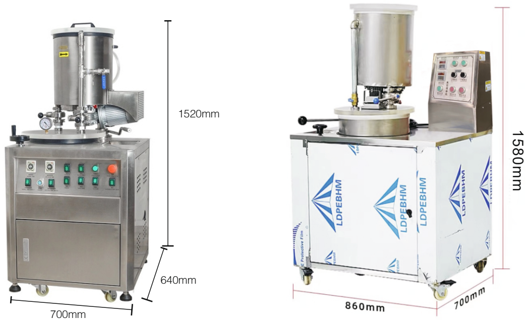
KYG0624 5盅真空搅拌机 (泵外置) 5Pcs Flask Vacuum Mixer Size:700x640x1520mm
