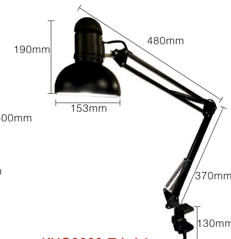
KYG0060 黑色台灯 Table-Stand Lamp(Black) Weight:870g 包装size:390x195x88mm
