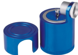
KYG0292 钻石腰码镜 Diamond Waist Size Loupe Size: \phi 42 H:68mm Weight:122g
