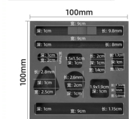
KYG1533 11孔石墨槽
