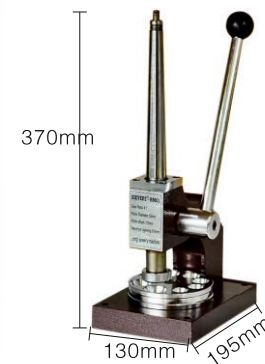
KYG0325 戒指扩大器 Ring Stretcher Weight: 12kg 机身尺寸(Dimension): 130 × 185 × 370mm 包装尺寸(Packing Size): 405 × 235 × 195mm
