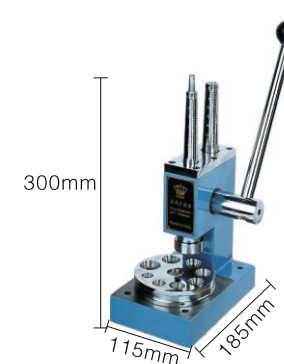
KYG0326 戒指扩大器 Ring Stretcher Weight: 8kg 机身尺寸(Dimension): 115 × 185 × 300mm 包装尺寸(Packing Size): 185 × 230 × 400mm
