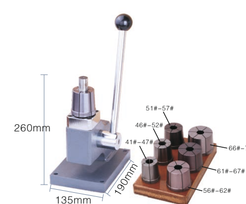
KYG0332 手镯扩大器 Bracelet Stretcher 机身尺寸(Dimension): 135 × 190 × 260mm 包装尺寸(Packing Size): 190 × 290 × 330mm Weight: 16 kg 可调范围(Adjustable extent): 41-72mm
