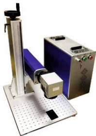
KYG0773 光纤激光打标机 Fiber Laser Marking Machine 支架尺寸: 400 × 600 × 550mm 机箱尺寸: 210 × 450 × 540mm Weight: 50kg
