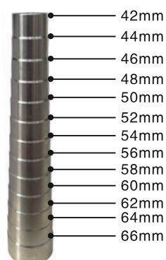
KYG0887 不锈钢实心手镯棒 Stainless Steel Solid Bracelet Mandrel H: 330mm Weight: 6.06kg
