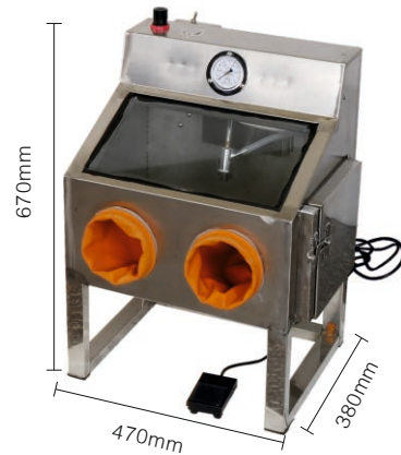
KYG0180 304不锈钢壳喷砂机 Dry Sandblaster Size: 470 × 380 × 670mm 304 Stainless Steel Shell Weight: 15kg
