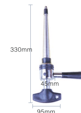
KYG0334 戒指扩大器 Ring Stretcher 机身尺寸(Dimension): 45 × 95 × 330mm 包装尺寸(Packing Size): 130 × 185 × 370mm Weight: 1.2kg
