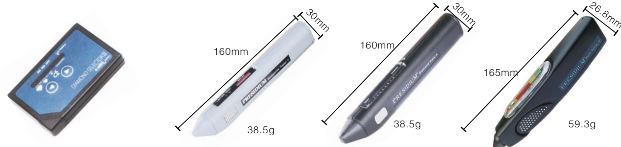
KYG0239 测石笔 Diamond Tester 包装Size:85 × 55 × 15mm
