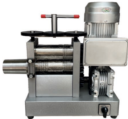
KYG0827 台式电动压片机(有拉线器) Electric Rolling Mill 电压(Voltage): 220V 功率(Power): 750W 滚轴直径(Roller Diameter): 68mm \times 160mm 长方槽(Cuboid): 1.5/2/2.5/3/4/5.5/7mm 半圆槽(Semicircular Groove): 5/6/7/8/10mm 压片宽(Width of Pressing Surface): 65mm 机身尺寸(Size): 400 \times 200 \times 490mm Weight: 50kg
