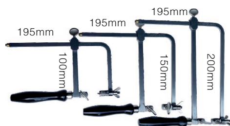
KYG1010 德国NIQUA牌锯弓 Germany NIQUA Brand Saw Bow No: 80mm/100mm/150mm/200mm Made in Germany
