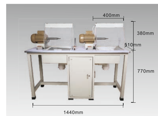
KYG0766 双位吸尘打磨机 Double Ended Polishing Machine 打磨功率Power: 550W × 2 吸尘功率Polishing power: 750W 电压Voltage: 220V 重量Weight: 90kg
