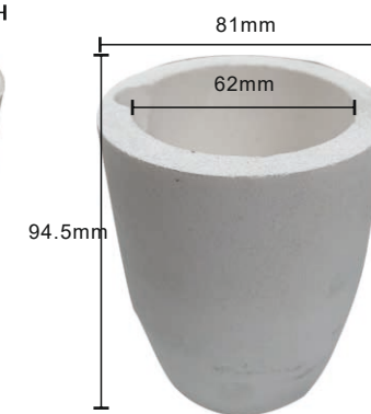
KYG1547 石英熔金坩 Ceramic Melting Crucible
