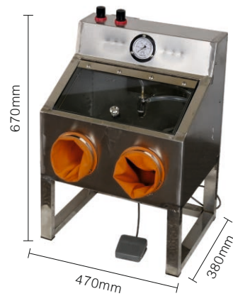
KYG0179 304不锈钢壳喷砂机 Wet Sandblaster Size: 470 × 380 × 670mm 304 Stainless Steel Shell Weight: 15kg
