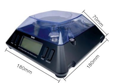
KYG0214 TANITA KP-601 克拉秤(双显示屏) Diamond Carat Scale NO.100g/0.002g 500ct/0.01ct 包装Size:225×280×105mm Weight:1.25kg Made In Japan
