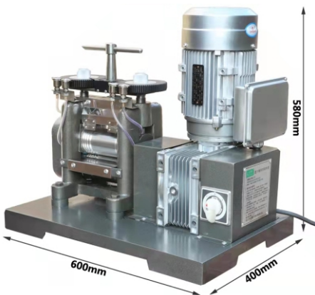
KYG0824 台式1.5匹电动压片机 Electric Rolling Mill 电压(Voltage): 220V 功率(Power): 1.5HP/1.1KW/220V 滚轴直径(Roller Diameter): 70mm \times 140mm 方槽(Square Groove): 0.8/1/1.2/1.5/2/3/4/5/6/7/8mm 压片宽度(Tablet Width): 75mm 机身尺寸(Size): 400 \times 600 \times 580mm Weight: 125kg
