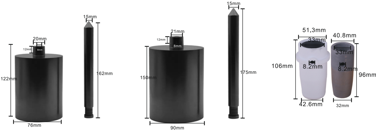
KYG1518 2kg倒模机熔金坩 Graphite Casting Crucible & Stopper 外 \phi 76x内 \phi 55xH122mm
