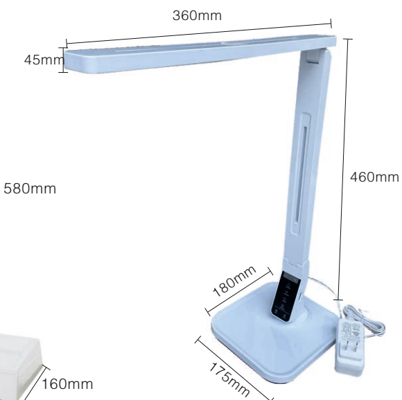
KYG0063 德国欧斯朗双管台灯 OSRAM Diamond Lamp 2 Tubes 机身Weight: 10kg 机身包装Packing Size 190*160*680mm 4pcs/ Carton Total Weight: 21.2kg Packing Size: 480*310*710mm
