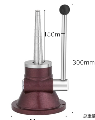
KYG0330 手镯扩大器(阶梯式) Bracelet Stretcher 机身尺寸(Dimension): 160 × 150 × 300mm Weight: 6kg 可调范围(Adjustable Extent): 52-70mm
