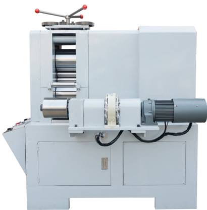
KYG0812 15匹精密四辊压片机 15P Four Rollers Precision Rolling Mill
