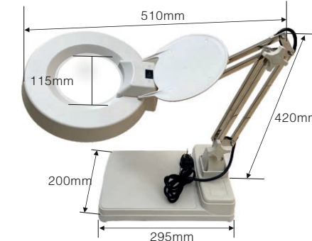
KYG0311 LED放大镜台灯 LED Magnifier Lamp Weight:2.94kg Magnify:10x 镜片尺寸(Lens size): 115mm 包装尺寸(Packing size): 30 \times 16 \times 39cm
