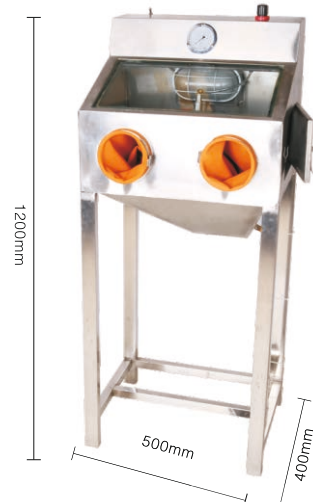
KYG0184 304不锈钢壳喷砂机 304 Stainless Steel Shell Sandblaster No1: 干喷 Dry Sand blaster No2: 水喷 Wet Sand blaster Size: 500 × 400 × 1200mm Weight: 17kg
