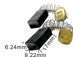
KYG0030 金科达SR碳刷 SR Carbon Brush 长度Length: 9.22 x 6.24 x 17mm 重量Weight: 3.2g
