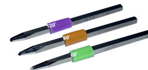
KYG0143 钨钢雕刻铲刀 Tungsten Steel Carving Shovel 型号: 60度/90度/120度 size: 2.32x2.34x54mm
