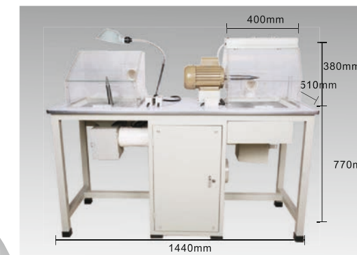
KYG0765 飞碟吸尘打磨机 Lapping & Polishing Machine 打磨功率Power: 550W × 2 吸尘功率Polishing power: 1100W 电压Voltage: 220V 重量Weight: 109kg
