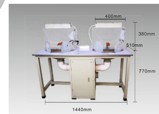
KYG0767 双位吸尘打磨机 Double Ended Polishing Machine 吸尘功率Polishing power: 750W 电压Voltage: 220V 重量Weight: 63kg
