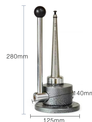
KYG0328 韩式单杆戒指扩大器 Ring Stretcher 机身尺寸(Dimension): 140 × 125 × 280mm Weight: 3.5kg
